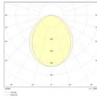
PC Opal diffuser-95°
