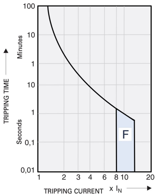
Tripping characteristic F
